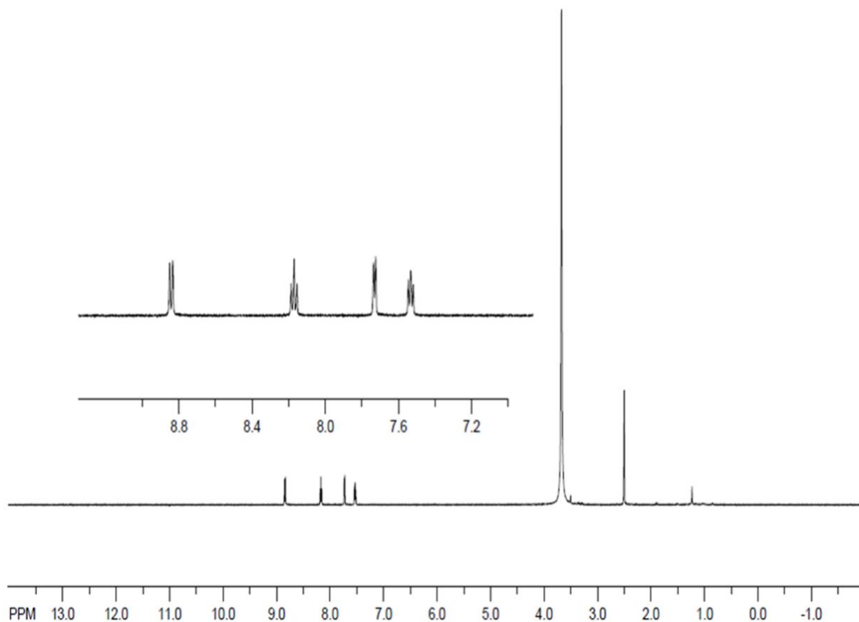
Figure 3 (a): 1 H NMR spectrum of the Ru [(bpy) 3 ] (Cl) 2 complex in the Me 2 SO-d 6 solvent at 298 K.
